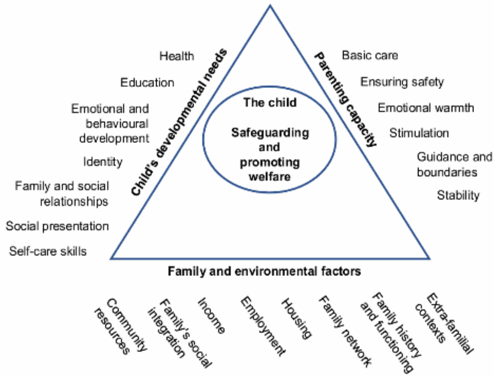
Figure 1: Assessment framework
